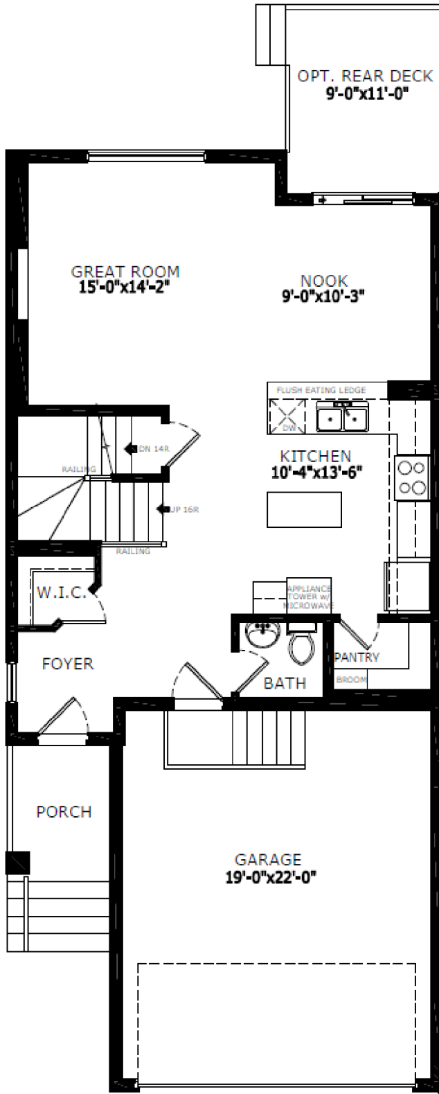
Main Level: 791 sq. ft.
