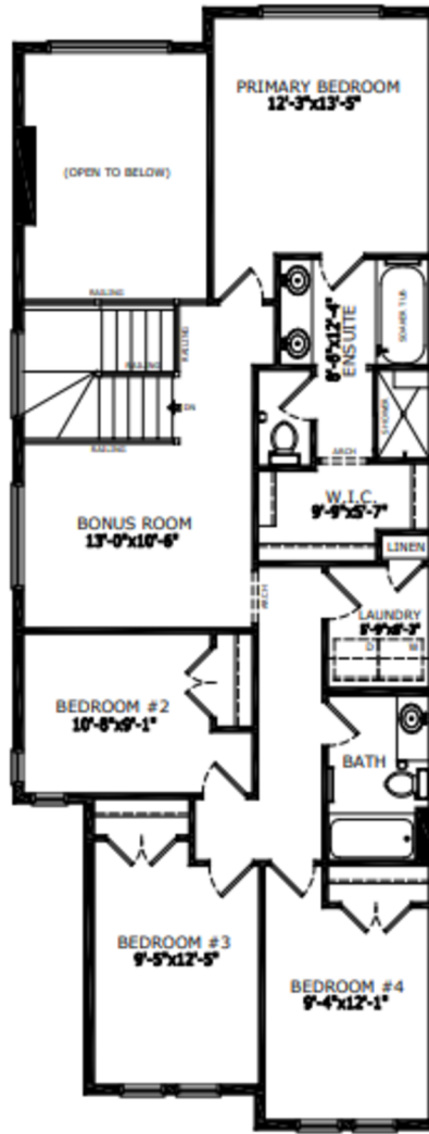
Upper Level: 1266 sq. ft.
