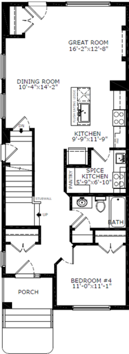
Main Level: 920 sq. ft.
