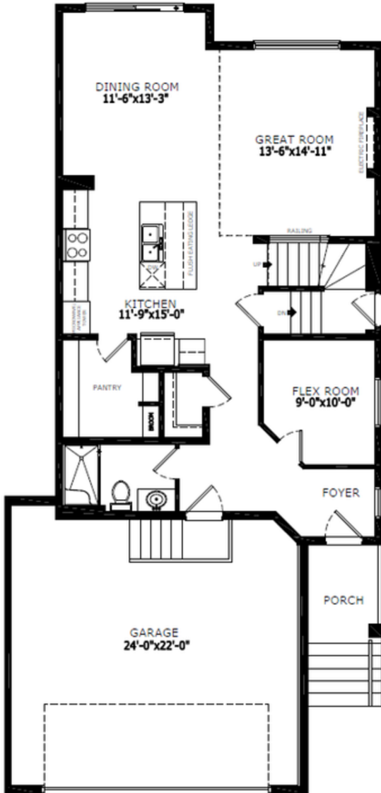
Main Level: 1039 sq. ft.
