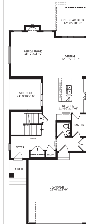
Optional Main Floor with Side Deck
