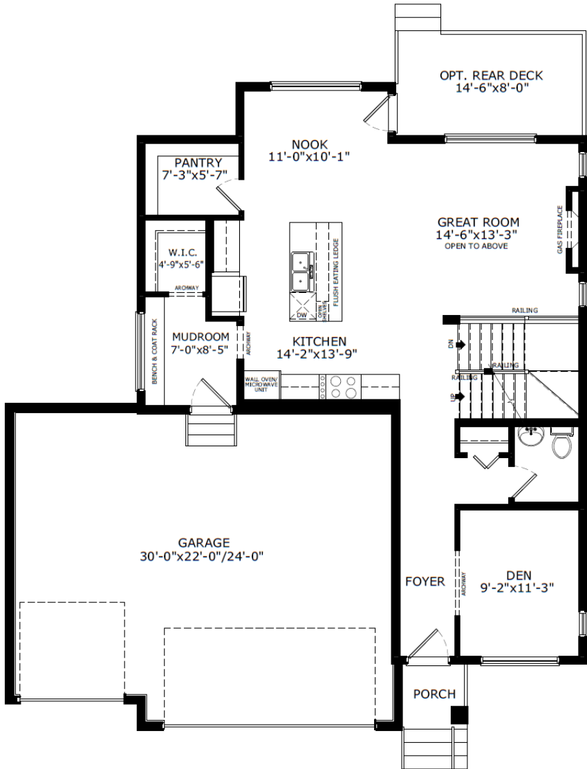
Main Level: 1041 sq. ft.
