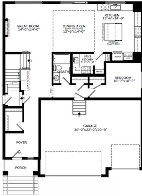
Main Level: 1302 sq. ft.
