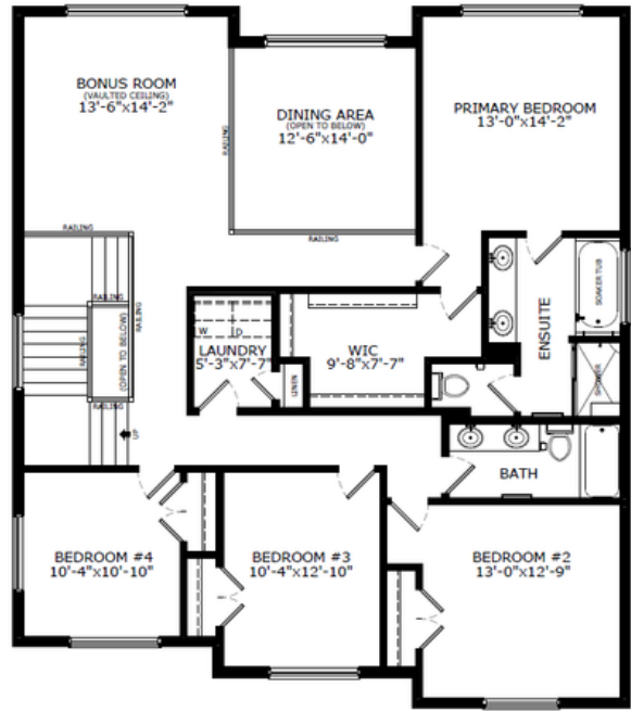
Upper Level: 1471 sq. ft.
