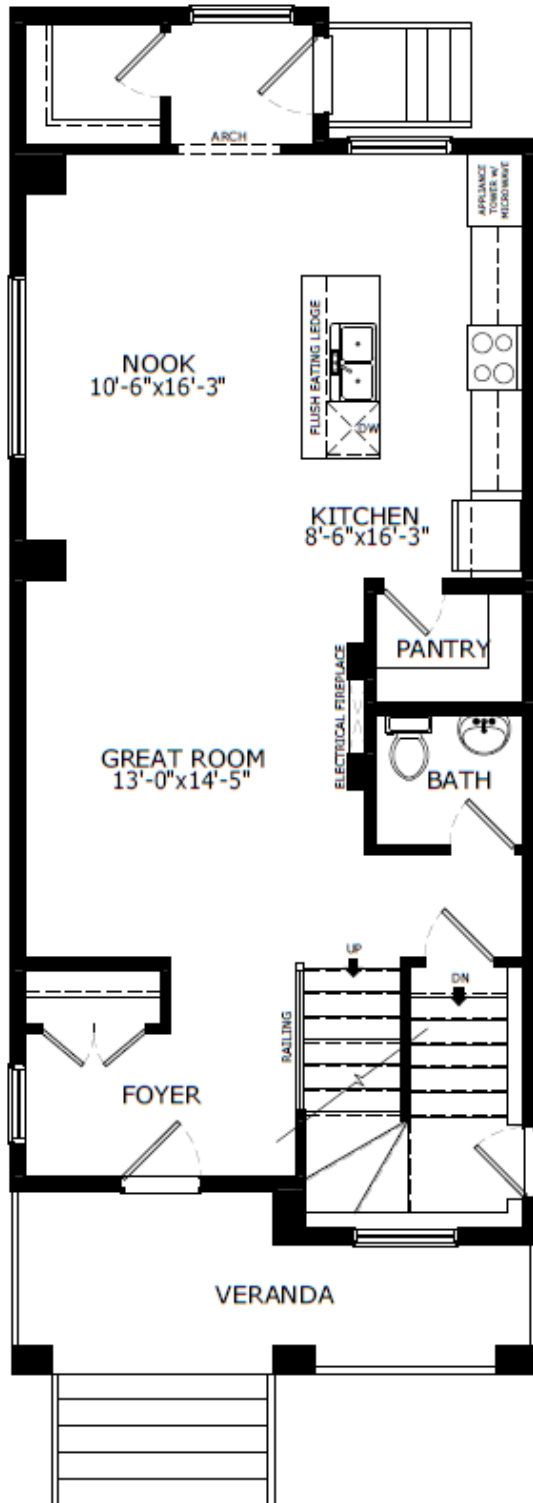
Main Level: 880 sq. ft.
