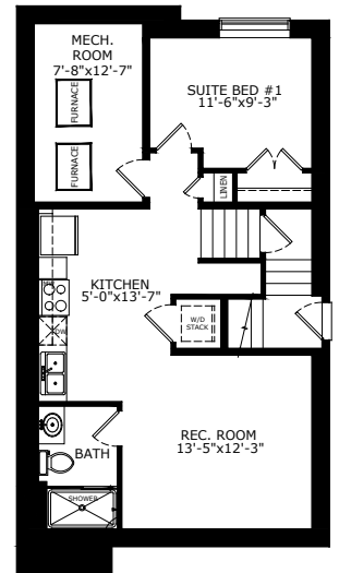
1 BEDROOM LEGAL SUITE - 574 SQ FT
