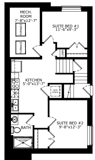
2 BEDROOM LEGAL SUITE - 574 SQ FT
