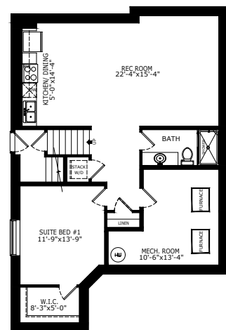
1 BEDROOM LEGAL SUITE - 848 SQ FT
