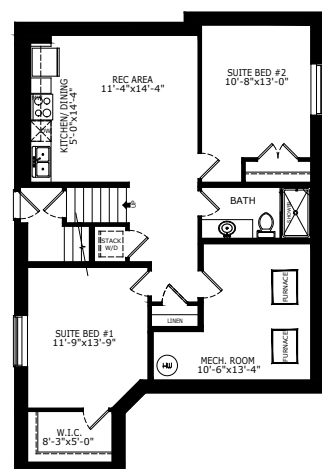
2 BEDROOM LEGAL SUITE - 848 SQ FT
