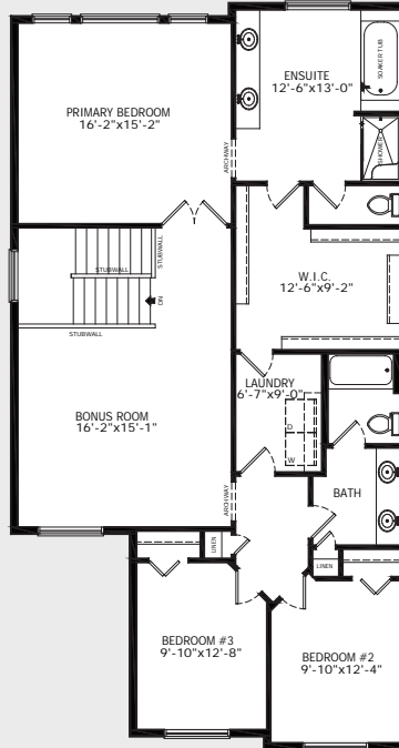
OPTION UPPER FLOOR PLAN - 3 BEDROOM WITH WALK THROUGH TO LAUNDRY
