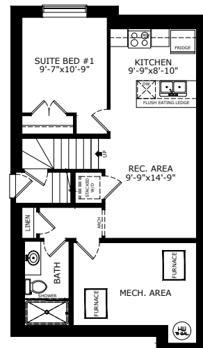
1 BEDROOM LEGAL SUITE - 531 SQ FT
