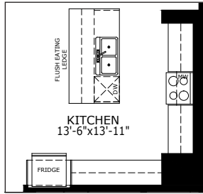
ALTERNATE KITCHEN #2
