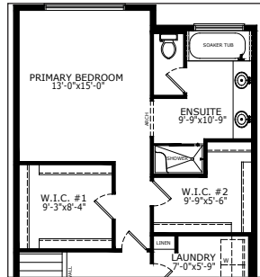
PRIMARY BEDROOM #1
