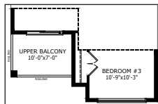
BALCONY
