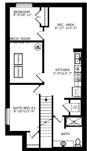
2 BEDROOM LEGAL SUITE - 766 SQ FT
