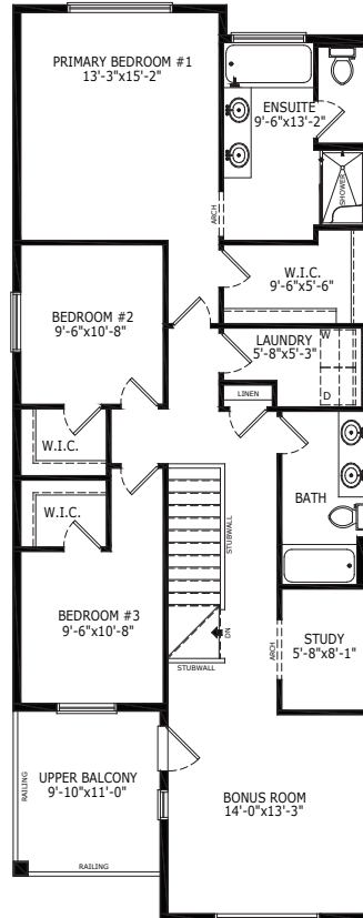
3 BEDROOM WITH BALCONY #2 - 1307 SQ FT
