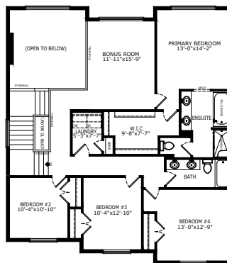
4 BEDROOMS WITH OPEN TO BELOW - 1513 SQ FT
