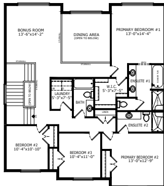
2ND PRIMARY BEDROOM 1558 SQ FT
