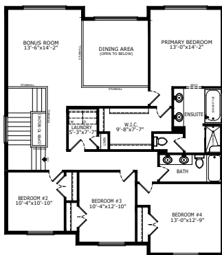
4 BEDROOM - 1558 SQ FT
