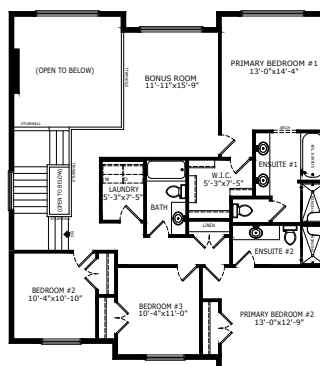
2ND PRIMARY BEDROOM WITH OPEN TO BELOW - 1513 SQ FT
