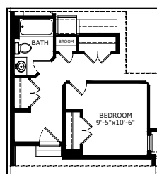
OPTIONAL FULL BATH WITH BEDROOM #1
