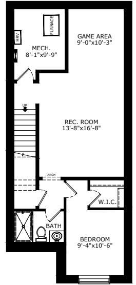
STANDARD - 629 SQ FT
