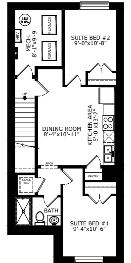
2 BEDROOM LEGAL SUITE - 631 SQ FT
