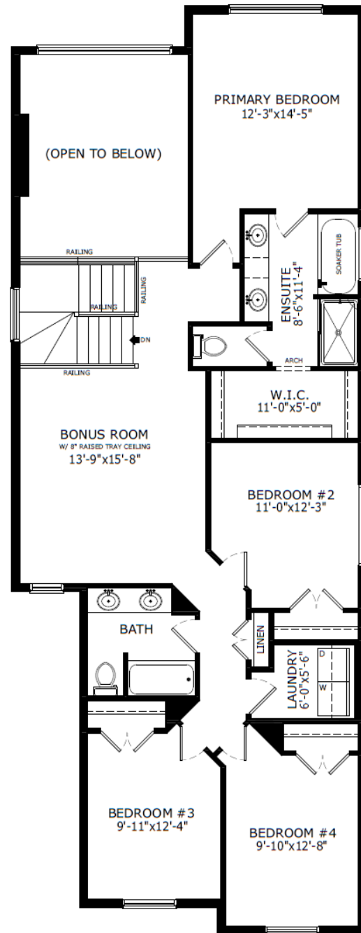
Upper Level: 1337 sq. ft.
