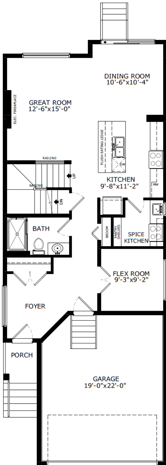
Main Level: 966 sq. ft.
