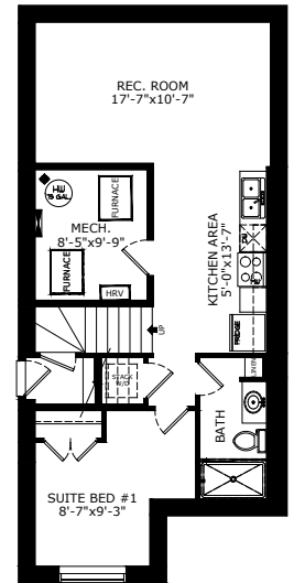
1 BEDROOM LEGAL SUITE - 583 SQ FT
