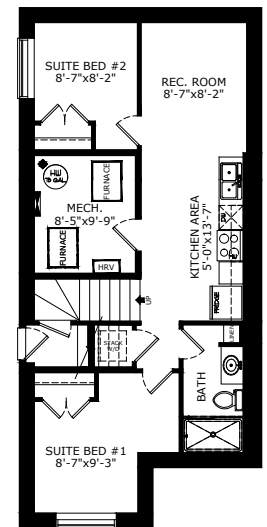
2 BEDROOM LEGAL SUITE - 583 SQ FT
